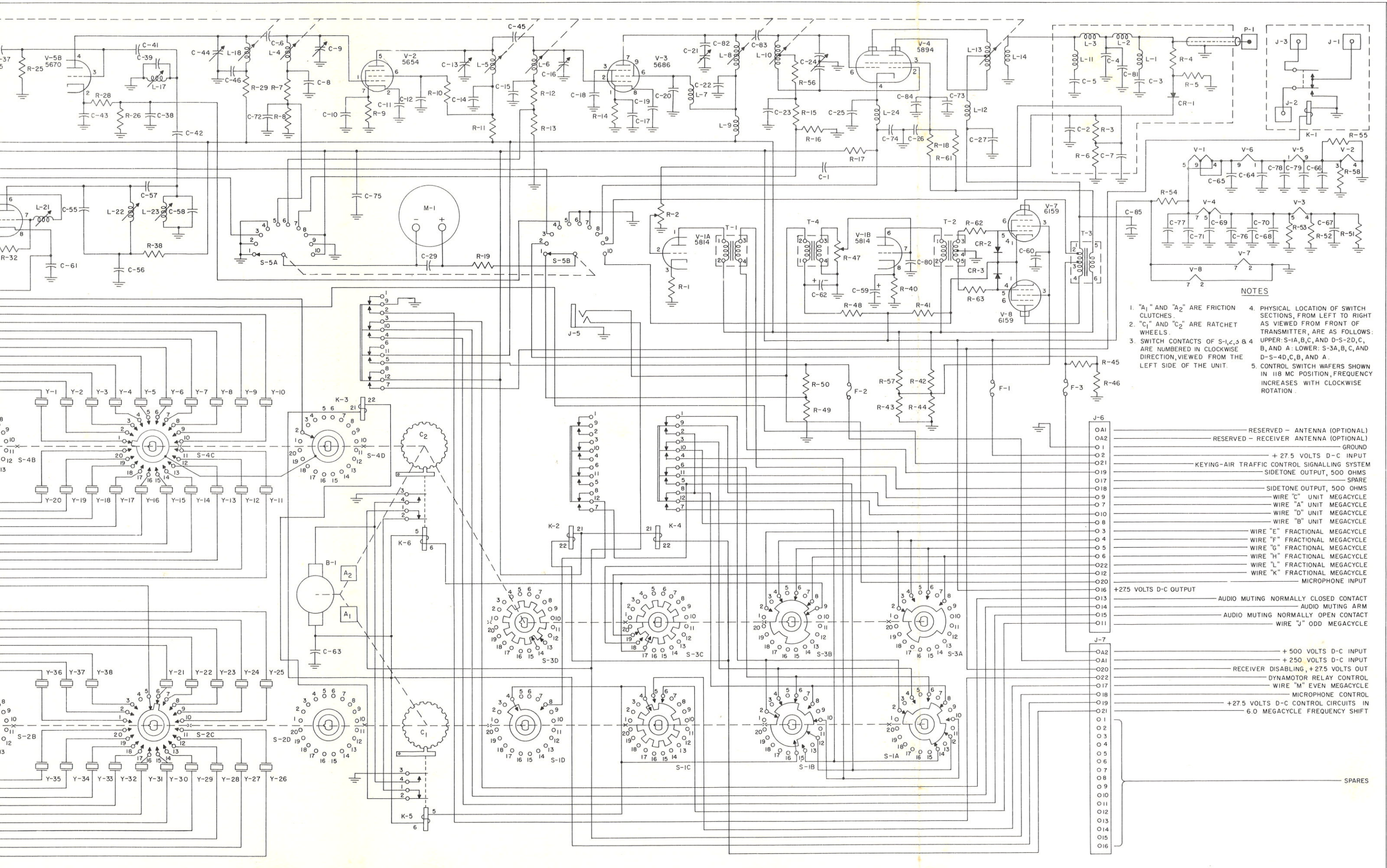
Figure 7-1. VHF Transmitter Series 707, Schematic Diagram
